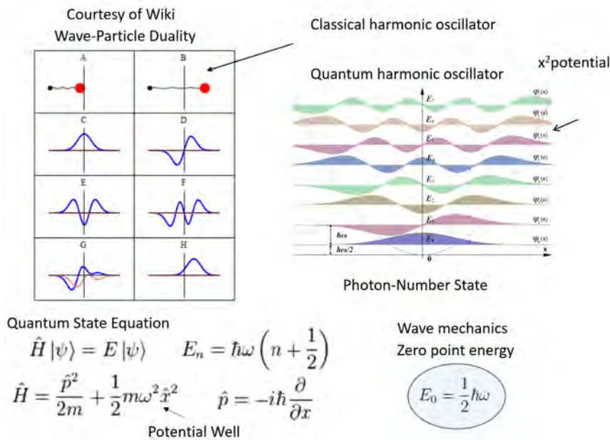
Figure 38.6: Plots of the eigensolutions of the quantum harmonic oscillator. The photon-number states are non-classical states because they do not have a classical analogue (courtesy of Wikipedia [285]).
