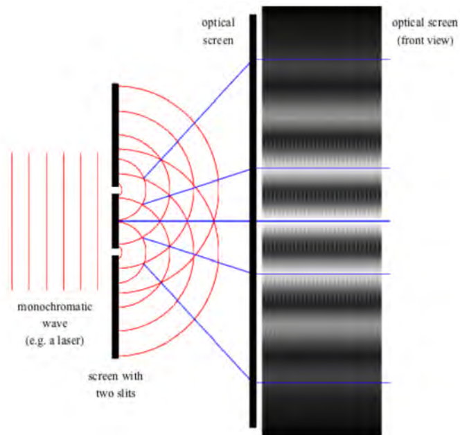
Figure 38.2: A Young's double-slit experiment. Again, the interference pattern reveals the wave nature of light (courtesy of [272]).
