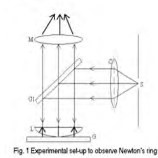
Figure 38.1: A Newton's rings experiment that indicates the wave nature of light (courtesy of [271]).
